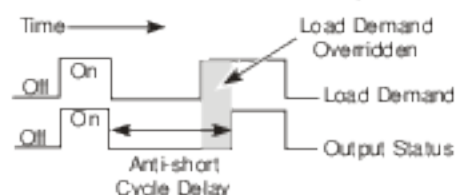
Figure 6: Anti-short Cycle Delay
