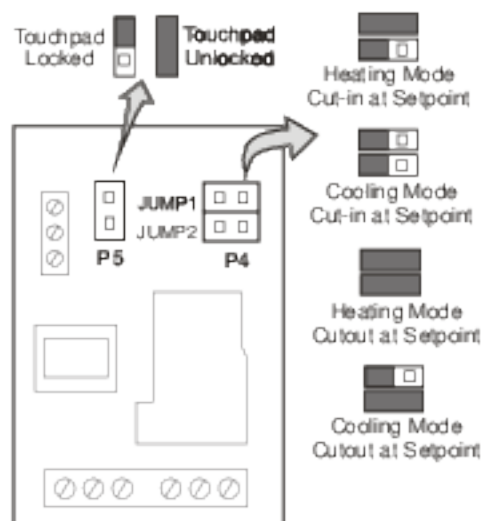
Figure 13: Jumper Positions and Control Settings
