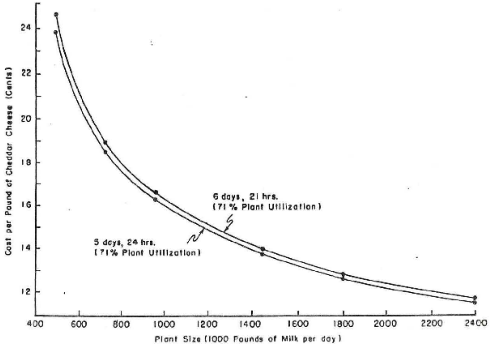
Figure 8. Average Production Costs for Different Size Cheddar Cheese Plants Using Automatic Cheddaring and 640/40-Pound Technologies, Operating Two Different Production Schedules with the Same Level of Plant Capacity Utilization.
