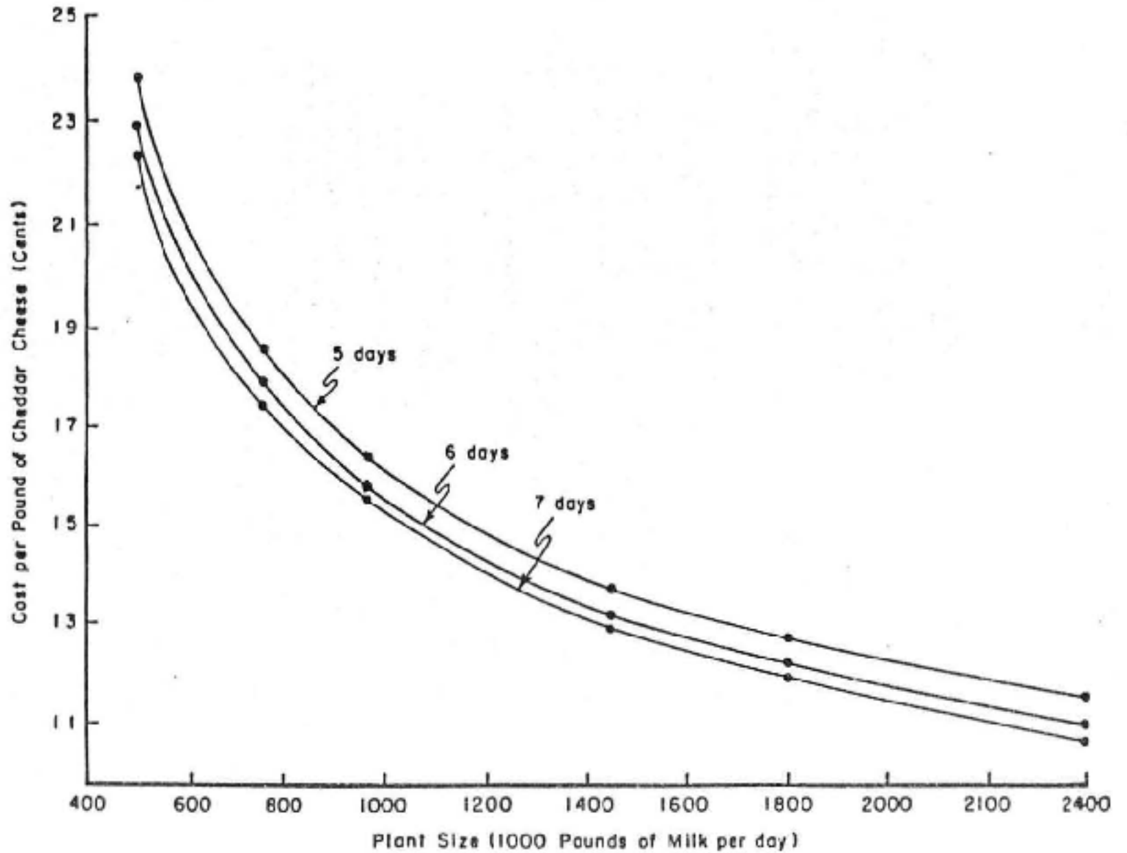
Figure 10. Average Production Costs for Different Size Cheddar Cheese Plants Using Automatic Cheddaring and 640/40-Pound Technologies, Operating 24 Hours per Day and Various Weekly Production Schedules.
