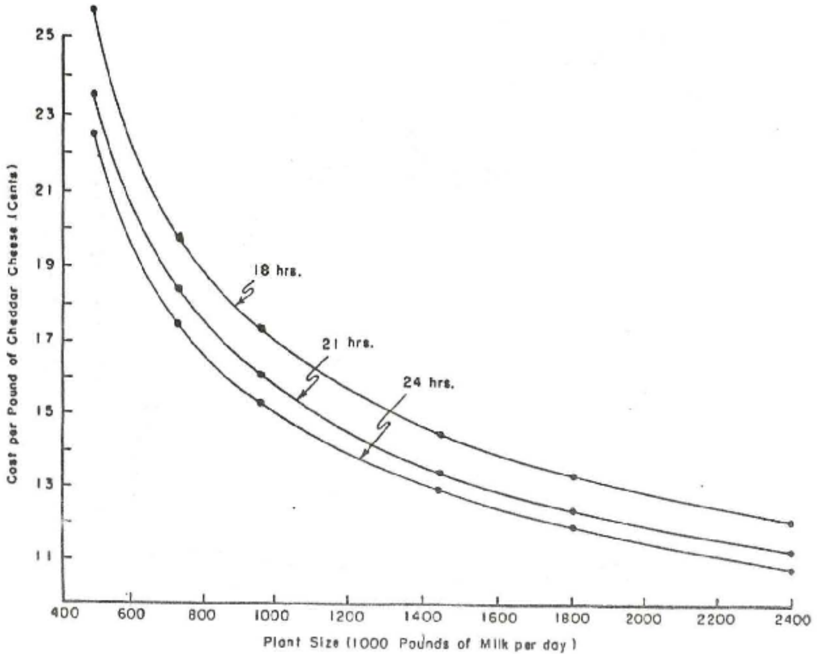
Figure 9 Average Production Costs for Different Size Cheddar Cheese Plants Using Automatic Cheddaring and 640/40-Pound Technologies, Operating 7 Days per Week and Various Daily Production Schedules.
