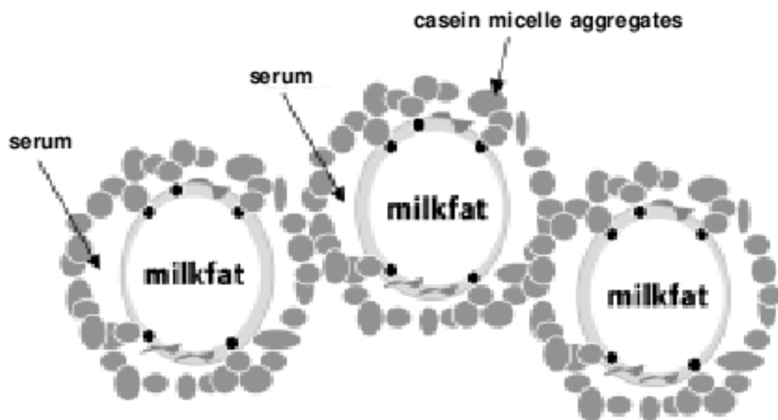
Figure 1. Casein micelles as an aggregate
