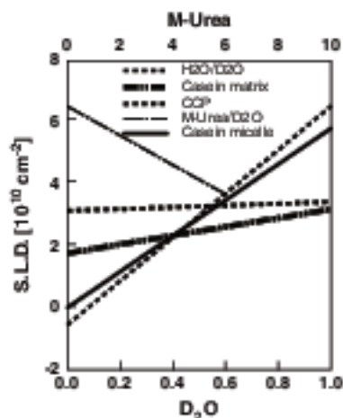
Fig. 1. The variation of the scattering length density of the protein, the colloidal calcium phosphate, the casein micelle particle and finally the contrast as a function of volume fraction of D 2 O on adding 6 MUrea to D 2 O contrast is lowered to 4 \cdot 10^{10} \text{ cm}^{-2} .
