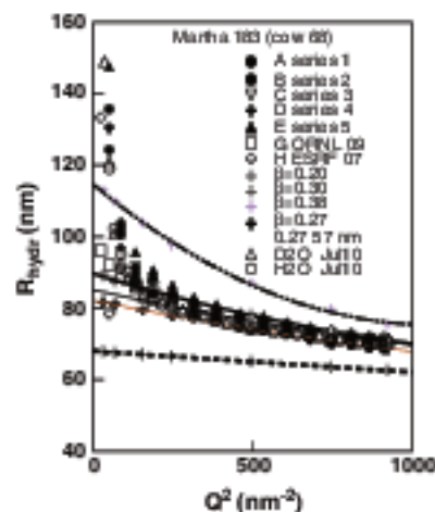
Fig. 6. Dynamic light scattering data for milk of cow 68 (Martha 183). Different milking over a period of 3 years. The drawn lines represent different degrees of polydispersity.
