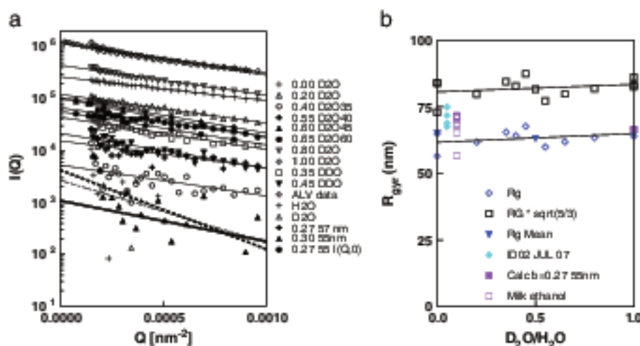
Fig. 7. a) Experimental Guinier plots at various D_2O/H_2O ratios. b) Calculated radius of gyration.
