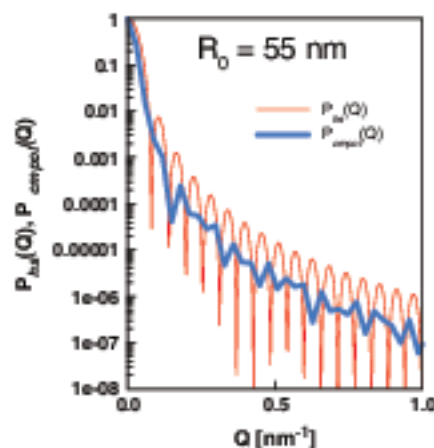
Fig. 5. Form factor, P(Q) (Eq. (8)) of a mono-disperse homogeneous sphere and the form factor of a collection of poly-disperse homogeneous spheres (Eq. (9)) R_0=55 \text{ nm} , \beta=0.27 , R_{\text{app}}=90 \text{ nm} , R_{\text{app}}(90^\circ)=80 \text{ nm} . The small fluctuations are due to numerical inaccuracies.
